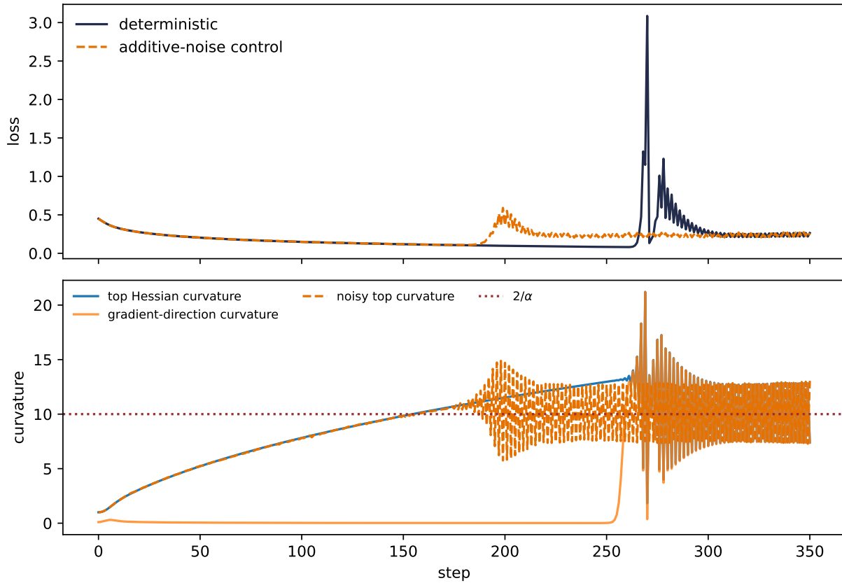
Figure 16.1.: A trajectory can begin below the quadratic stability edge and later move the local top curvature across it. A small additive-noise contrast preserves the crossing but shifts its timing and loss increments; neither trace turns a local quadratic threshold into a global divergence theorem.
