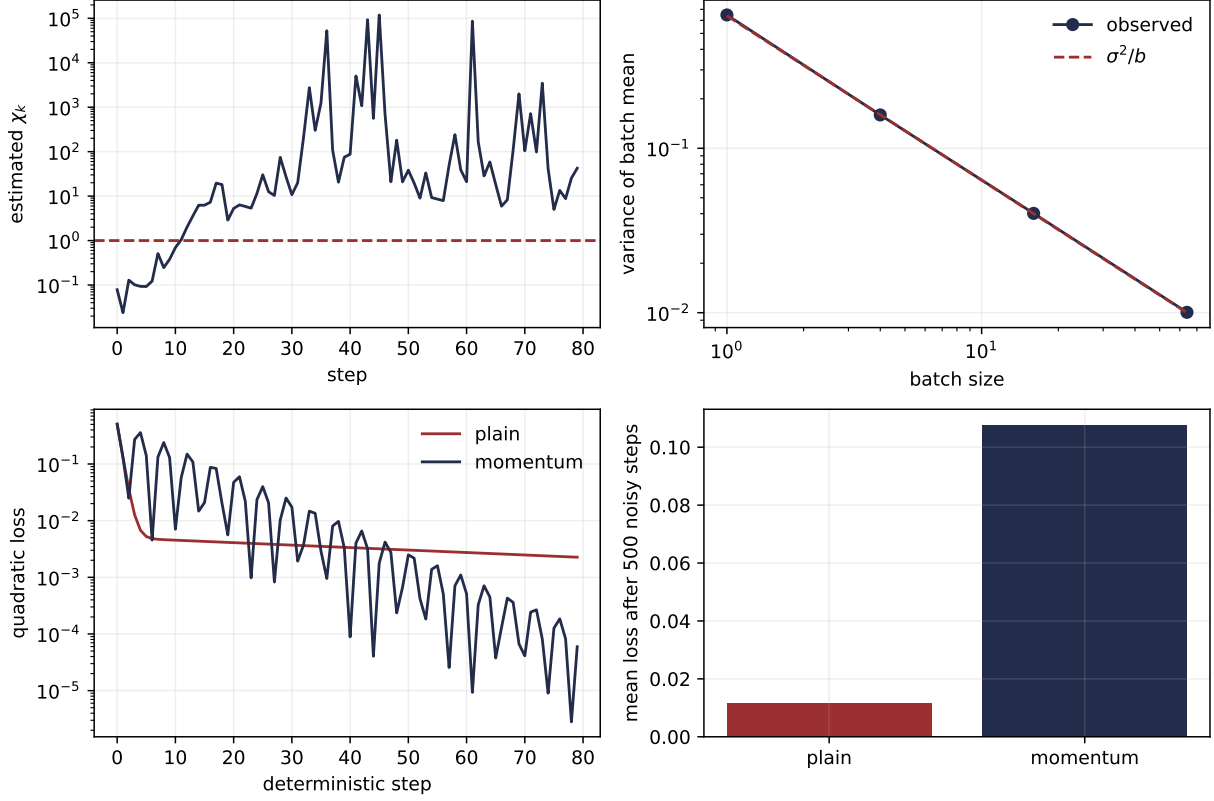
Figure 13.2.: Four controls separate four mechanisms. The online run crosses chi equals one with objective, step, noise scale, and batch fixed; independent batch means follow the one-over-b variance law; momentum improves the deterministic ill-conditioned control but amplifies shared stochastic forcing. The Pareto clipping calculation is reported separately because its variance is infinite.
