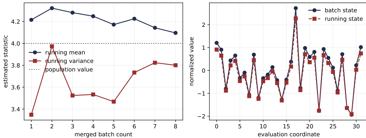
Figure 15.2.: Training and evaluation modes can disagree without distribution shift. The running state merges eight centered batch states exactly up to rounding, while the held-out batch has different finite estimates; normalizing the same evaluation values under those two states changes the outputs.
