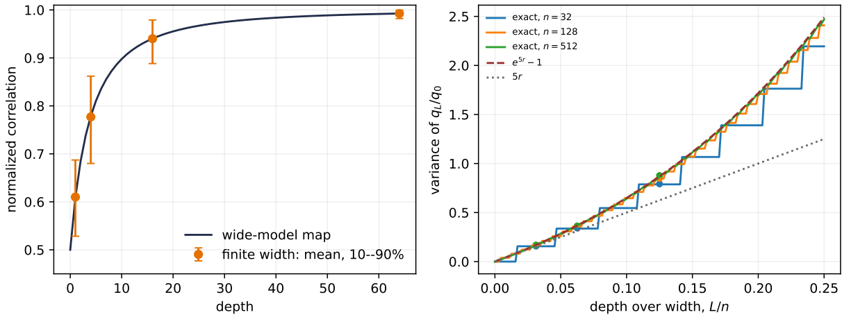
Figure 14.1.: Left: at critical ReLU scale, each input keeps its moment while two inputs align; finite-width means follow the wide correlation map. Right: the exact moment-fluctuation variance bends away from its 5L/n tangent as depth over width grows. The Monte Carlo points check the finite-width identity rather than replacing it.
