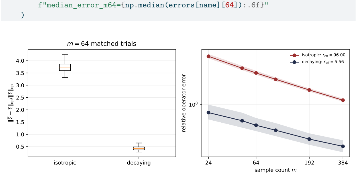
Figure 10.1.: Rank and top eigenvalue do not determine covariance-estimation difficulty. Both 96-dimensional populations are full rank with operator norm one. Their effective ranks are 96 and about 5.56. Across 300 matched Gaussian trials, the decaying-spectrum covariance has far smaller relative operator-norm error.
